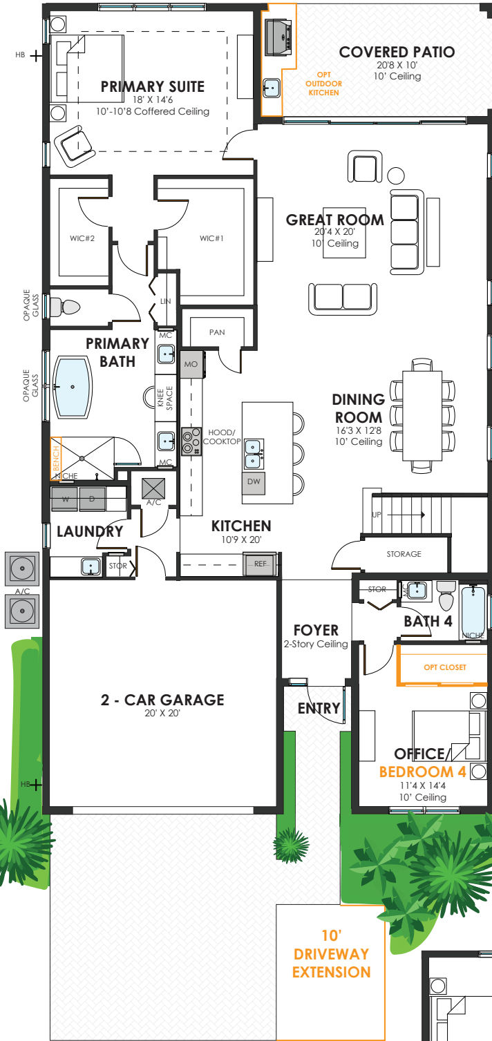
FIRST FLOOR
