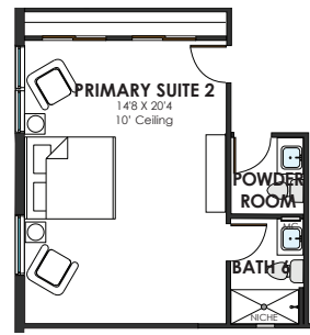
FIRST FLOOR SUITE 2 OPTION
